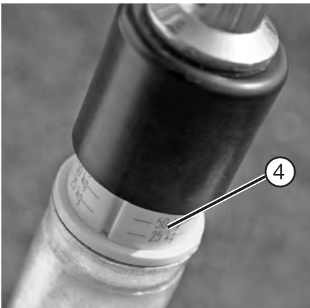
Drawbar load display on front landing wheel
