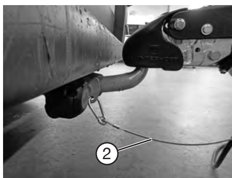
Rapid-emergency brake
