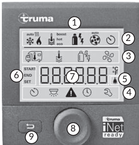
Truma control panel "CP plus"
